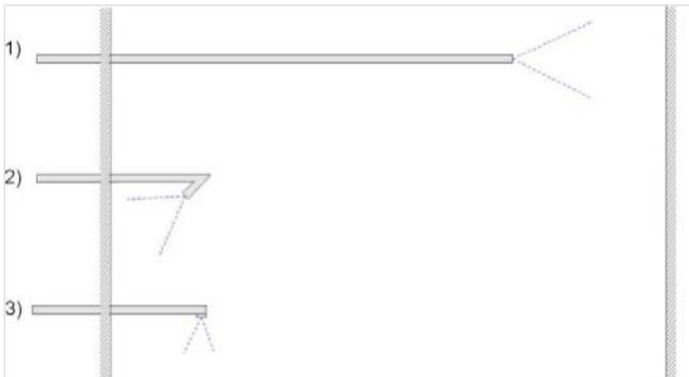
Figure 1 1) Long water-cooled video probe (up to 9 m) with field of view forward, 2) field of view of video camera backwards (to see slag deposits at burner) and 3) tilted field of view. Probe diameters typical 22-60.3 mm.
