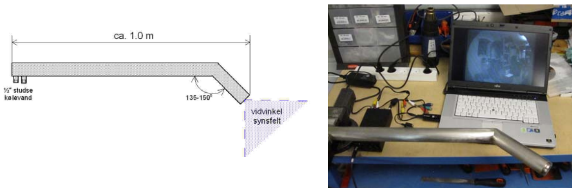
Figure 2 Popular simple water-cooled video probe with (tilted view) or without bend (looking forward) of probe. Probe diameters 22 mm, 32 mm, 45 mm or custom (e.g. 12 mm).
